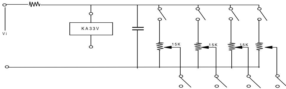
Figure 9. Electronic Tuner
