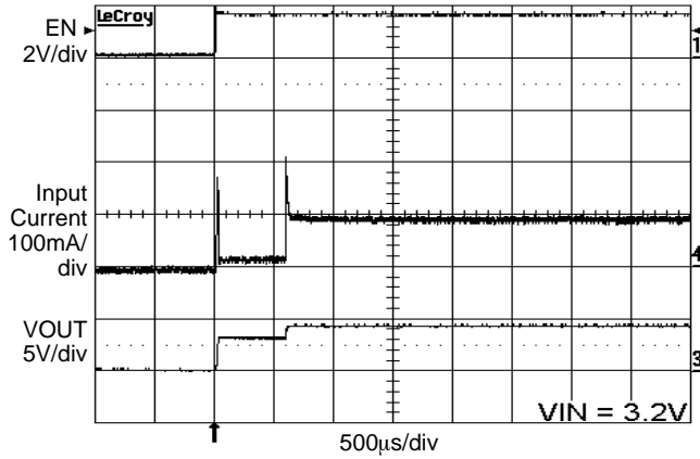
Figure 16. Power Up 3 LEDs at 20 mA, VIN = 3.2 V (1.5x Mode)
