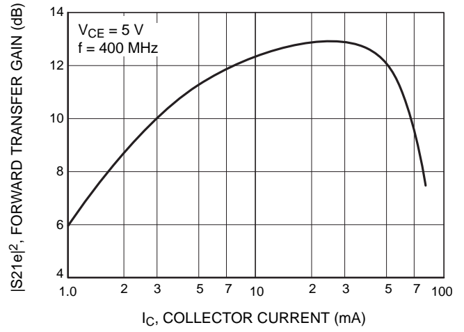
Figure 8. |S_{21e}|^2 – I_C
